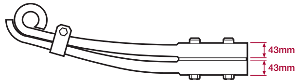
Type 3 : Current Spring
