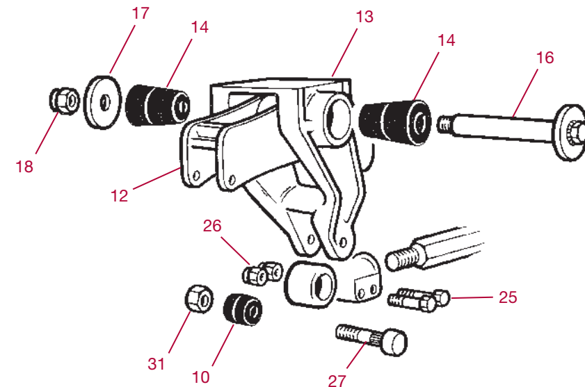
Hanger Bracket Assembly
