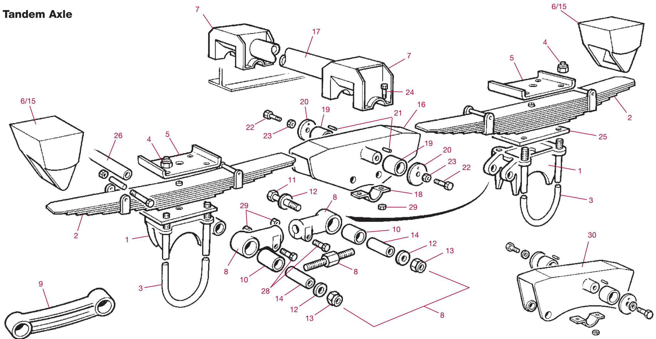
Rocker - Early Design
