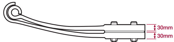
Type 1 : Early Spring (Obsolete)
