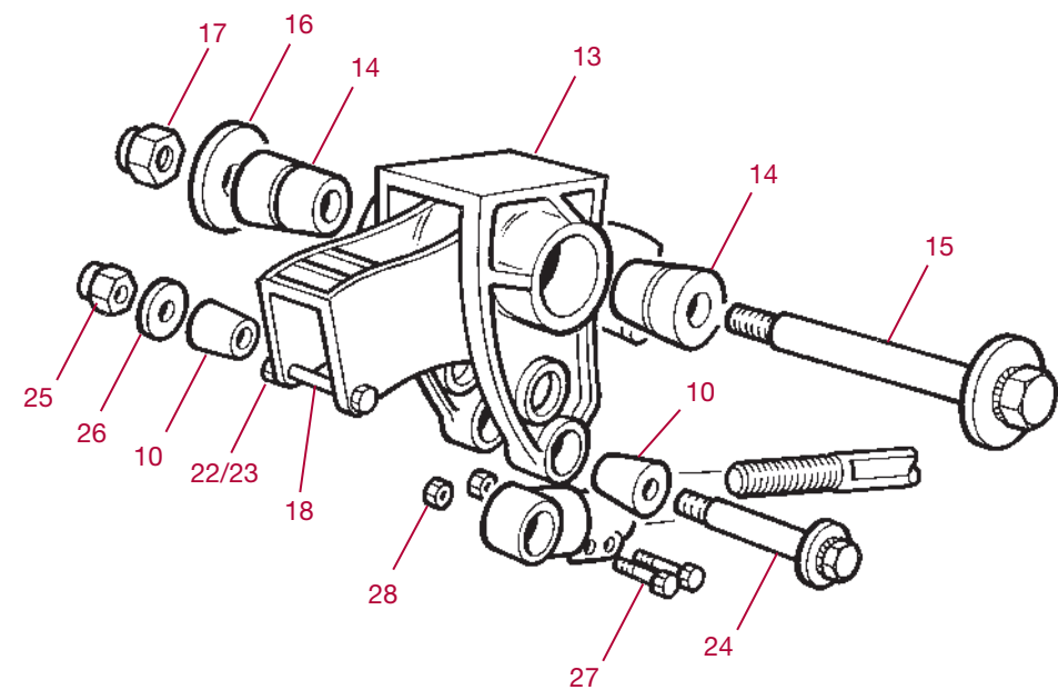
Hanger Bracket Assembly
