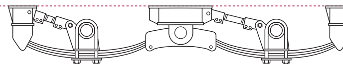
Semi-Wide Tandem Axle
