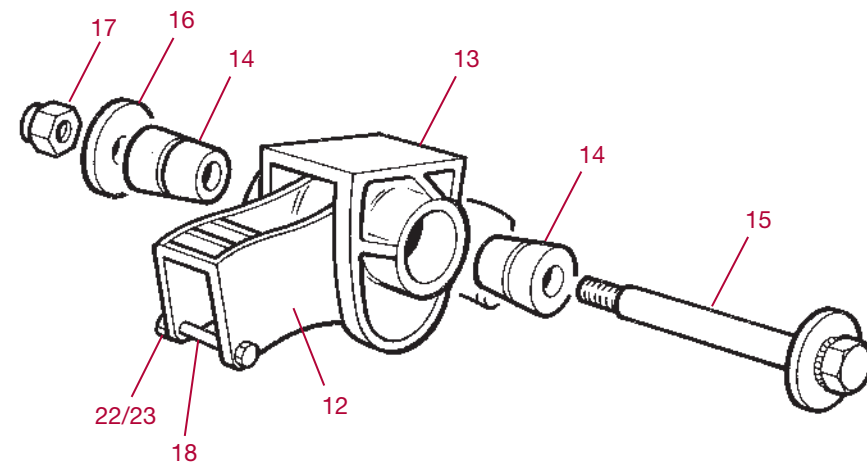
Rocker Bracket Assembly
