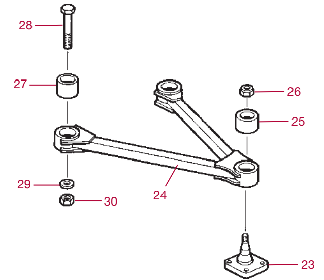
Torque Rod Assembly
