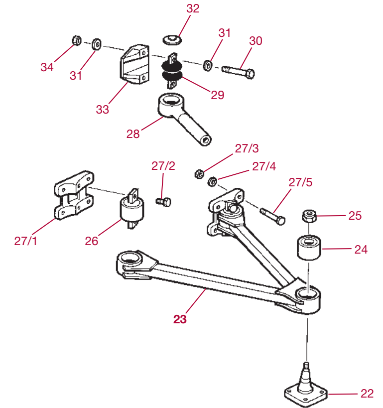
Torque Rod Assembly
