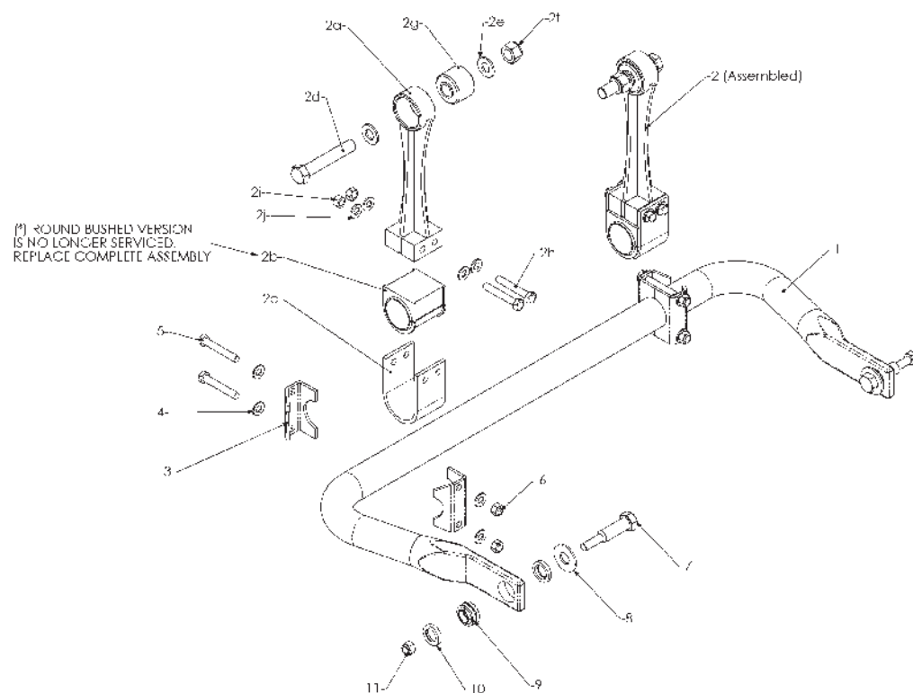
HNTRE - ANTI-ROLL BAR ASSEMBLY (EARLY ERF'S AND DENNIS EAGLE)
