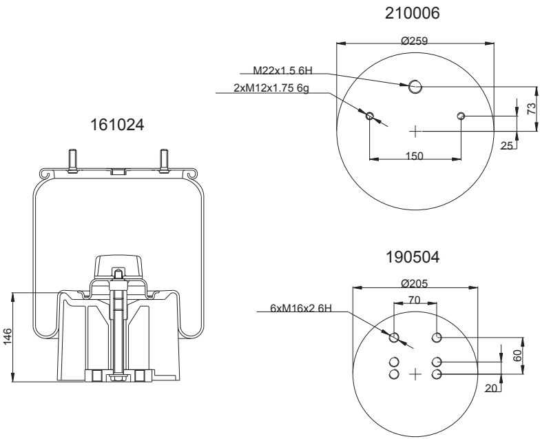
(Composite Piston)
