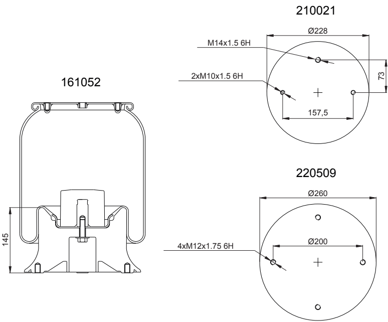
(Composite Piston)
