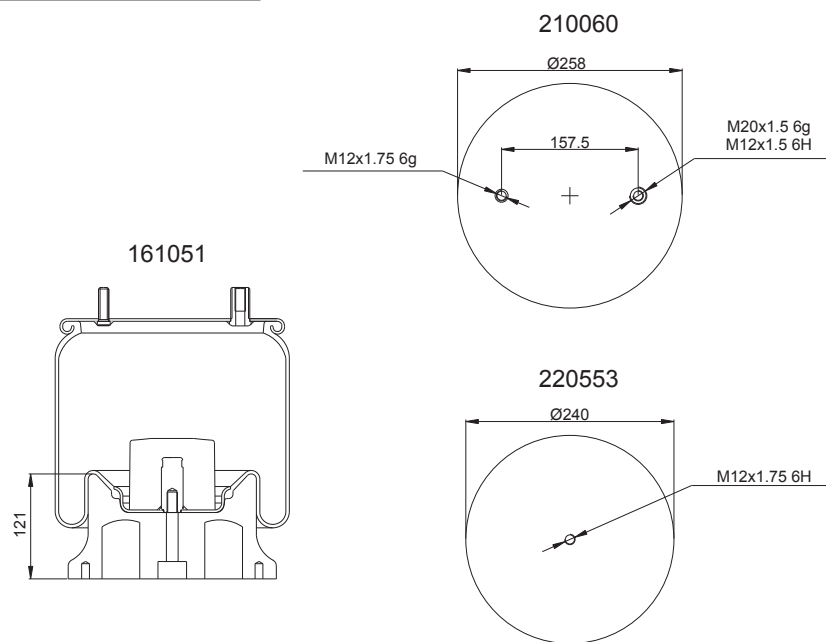
(Composite Piston)
