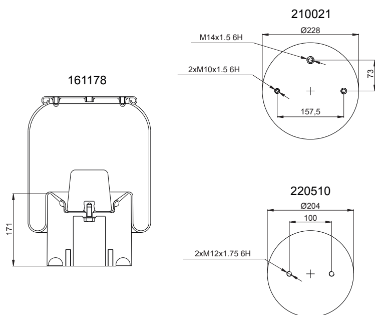
(Composite Piston)
