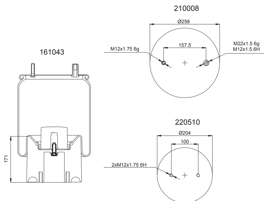
(Composite Piston)
