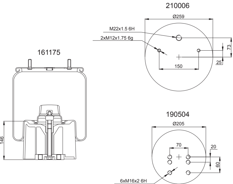
(Composite Piston)
