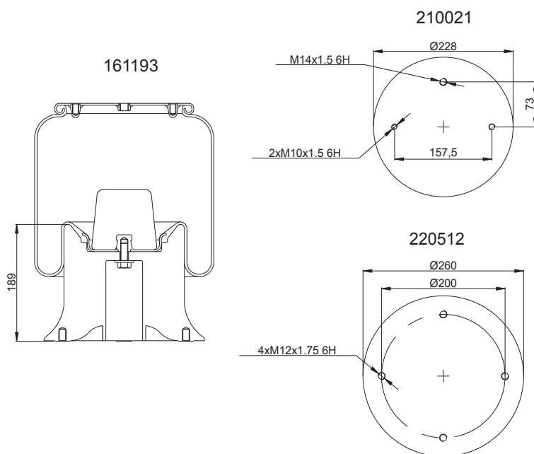
(Composite Piston)
