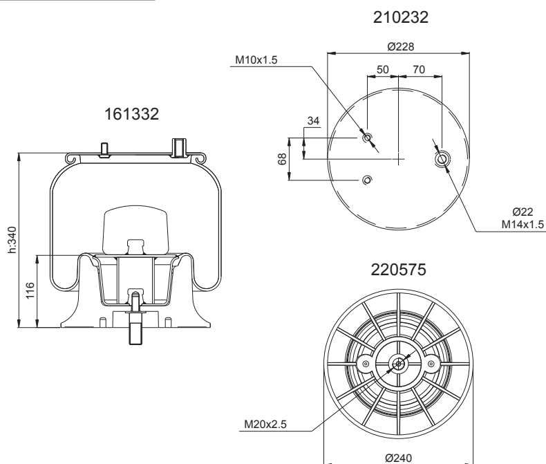
(Composite Piston)
