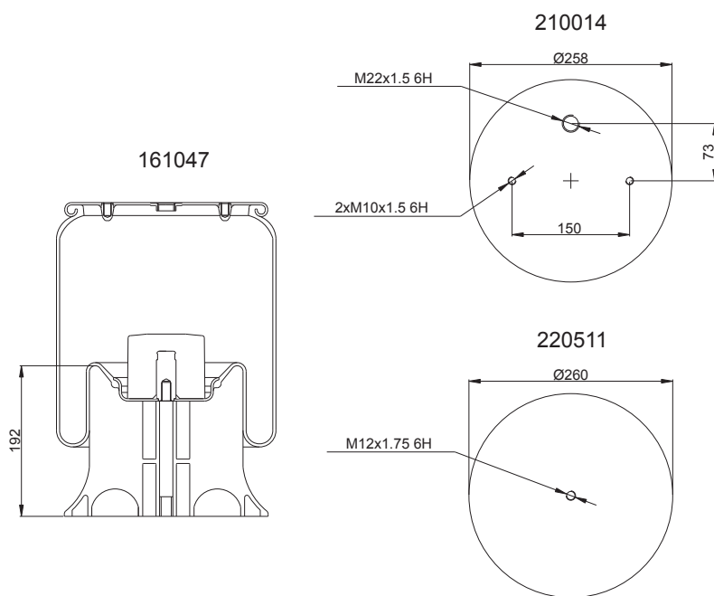
(Composite Piston)
