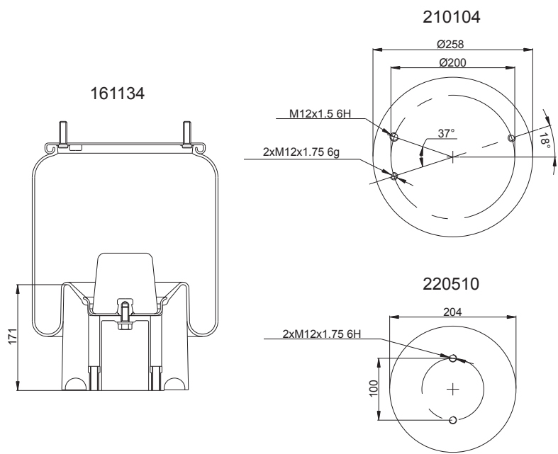
(Composite Piston)
