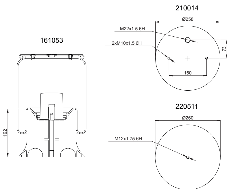
(Composite Piston)
