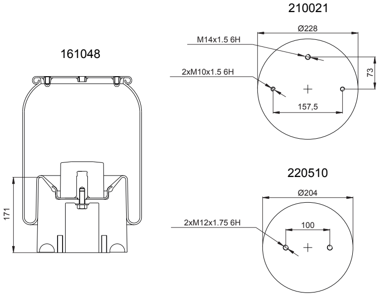
(Composite Piston)
