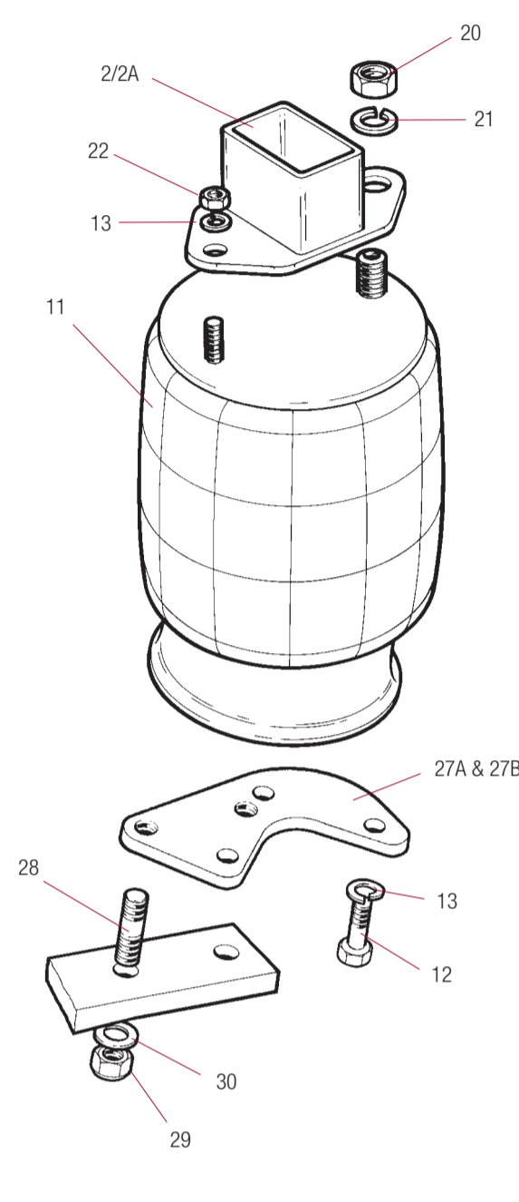
2 Stud Airspring and Offset Support Plate (handed) FL11000CS, FL11000LS & FL11000S
