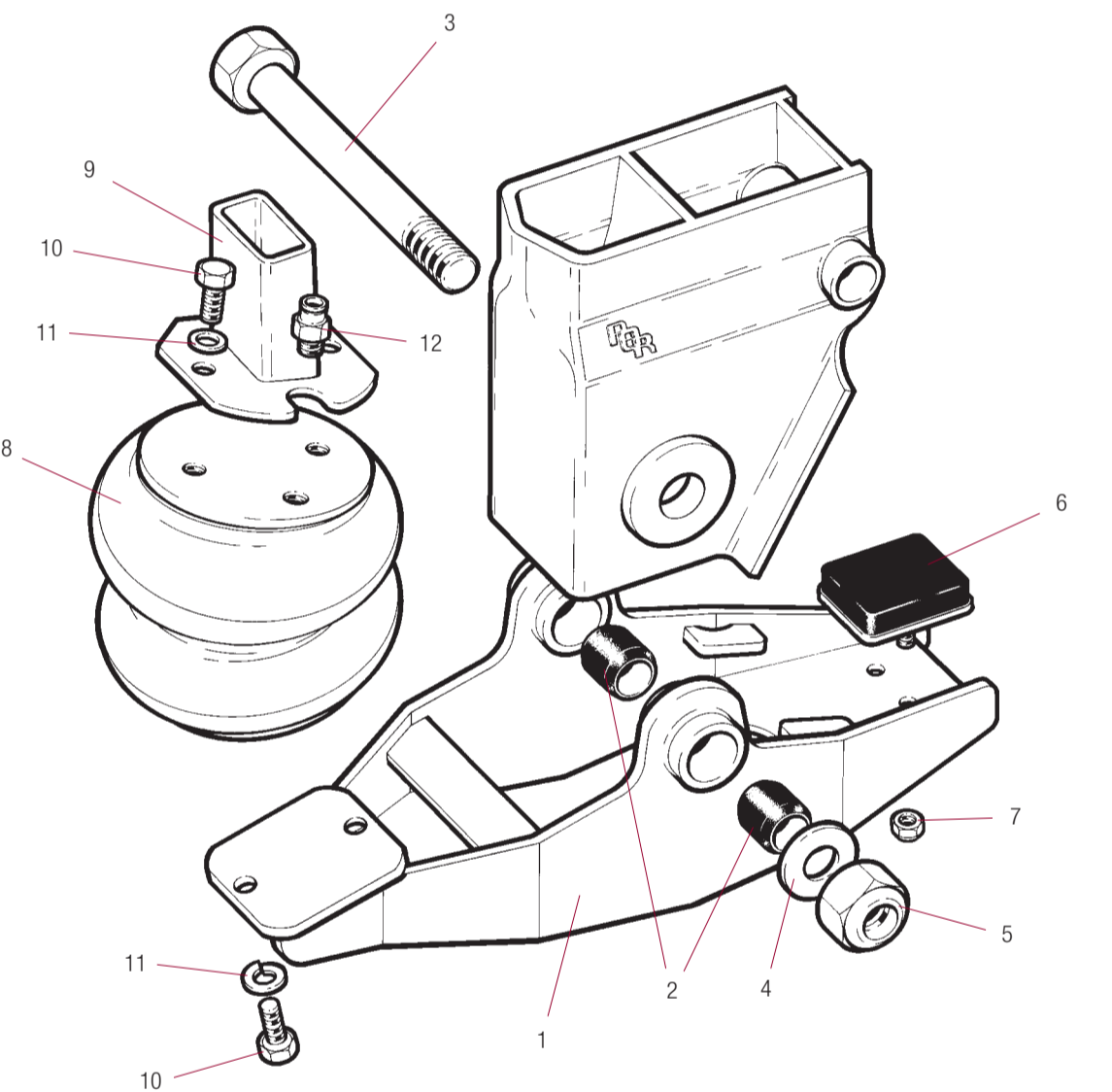
Axle Lift Suitable for use with FL11000 Suspensions M30 Kit No. 75223971 M24 Kit No. 75223971M24
